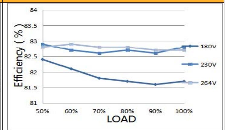
Fig.6 Efficiency-Load curve
